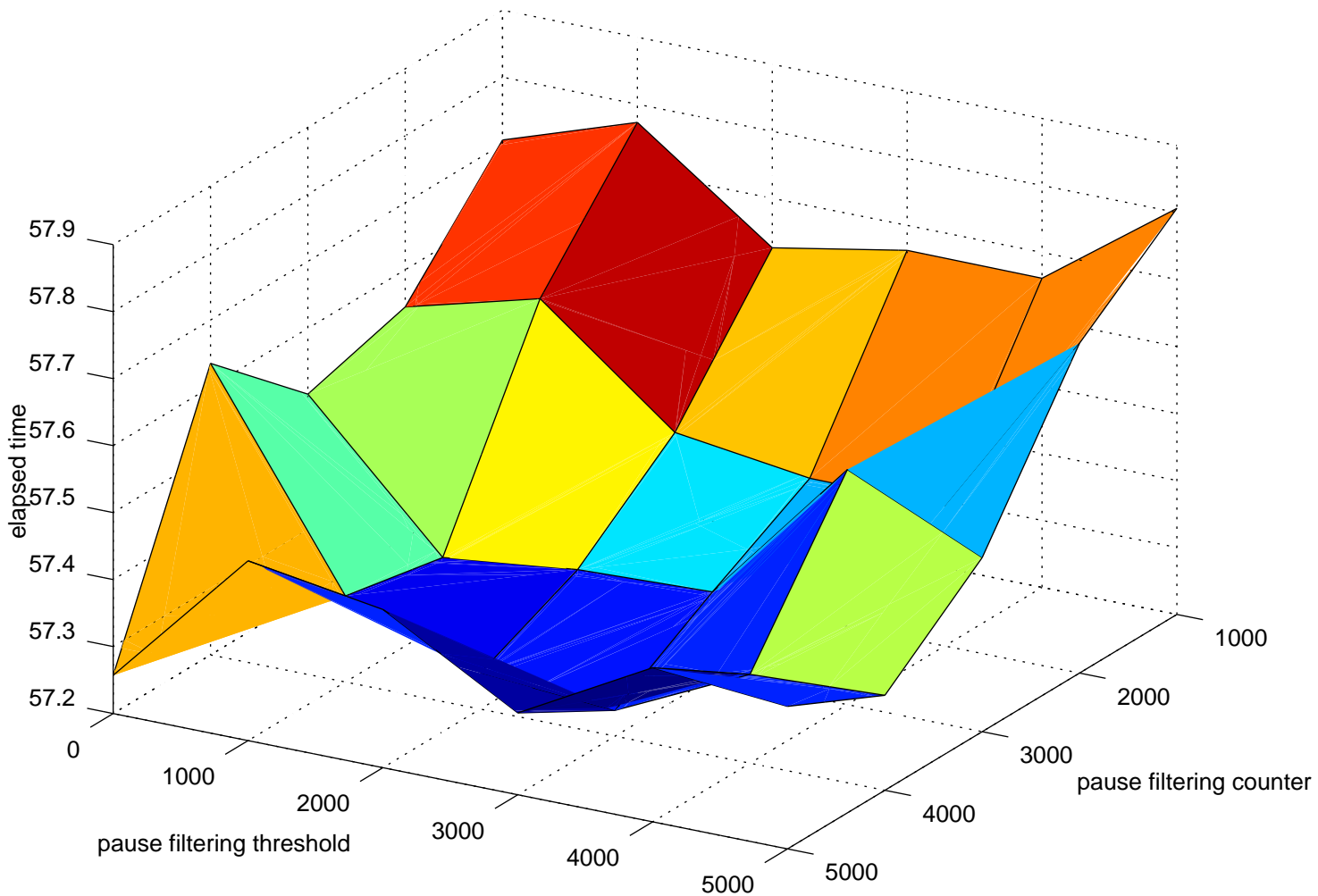
Elapsed time 24 pi test per VM vs pause variables
