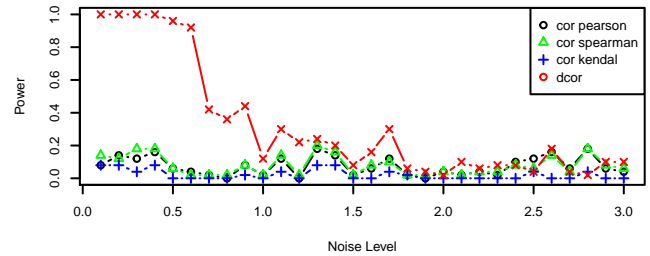
Sine: period 1/8
