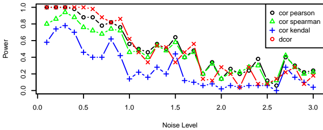
Sine: period 1/2
