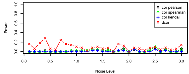
X^(1/4)
