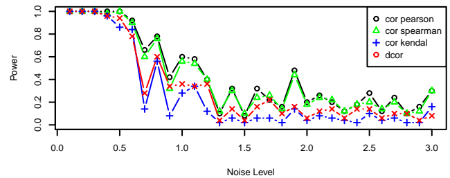
Step function
