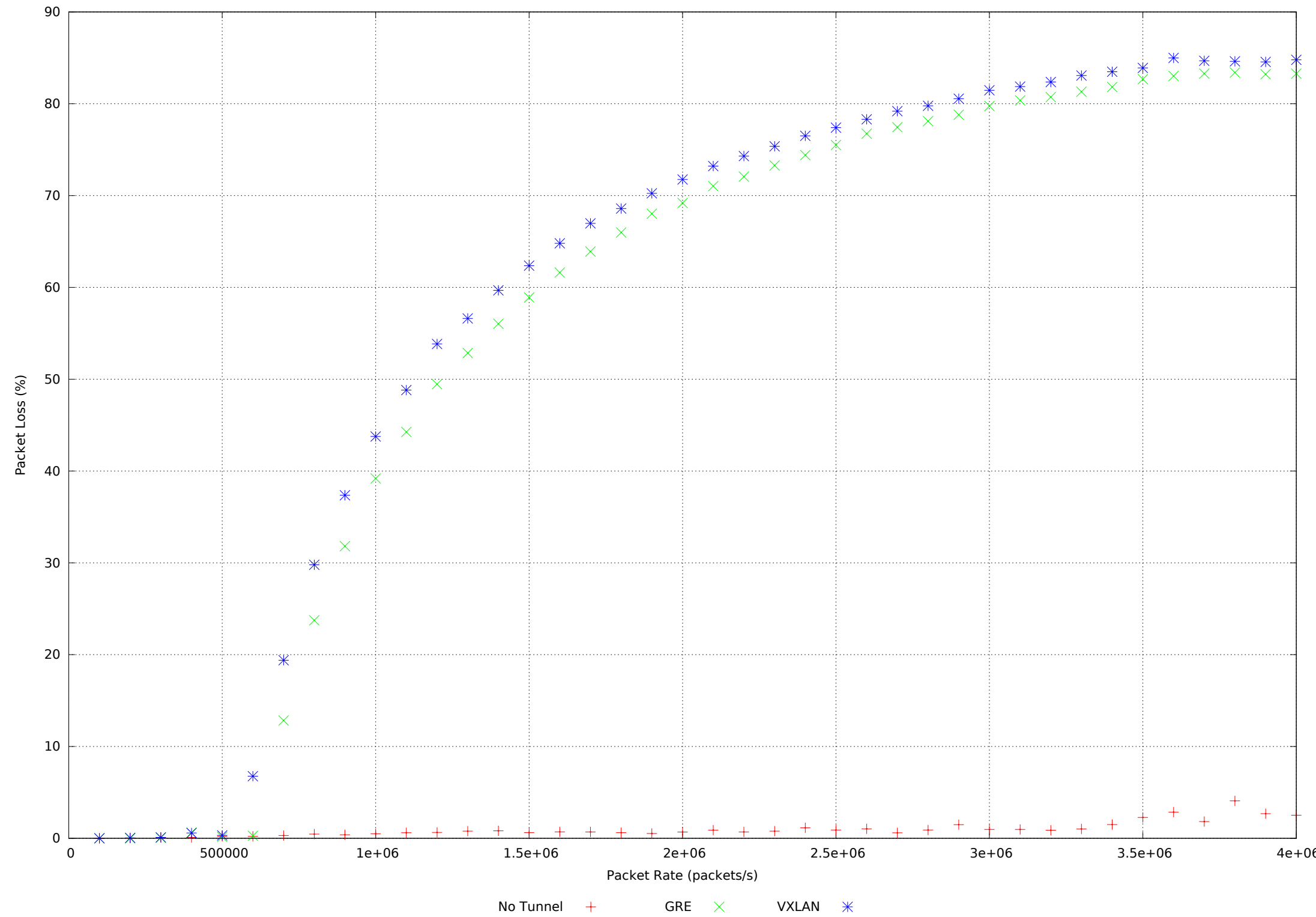
Packet Loss on Forwarding OVS Bridge vs Packet Rate - 96 Flows, 64Byte Packets
