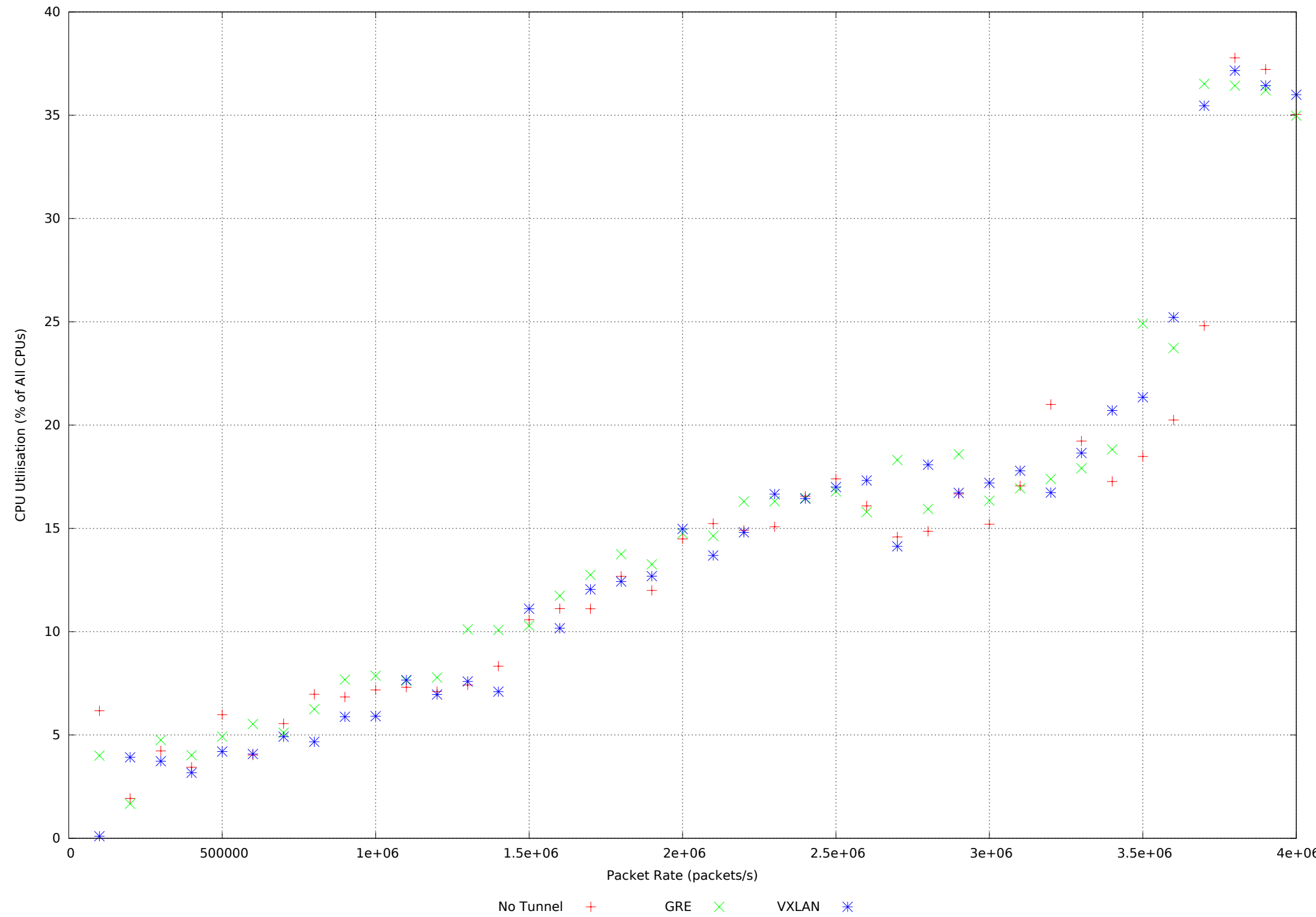
CPU Utilisation on Forwarding OVS Bridge vs Packet Rate - 96 Flows, 64Byte Packets
