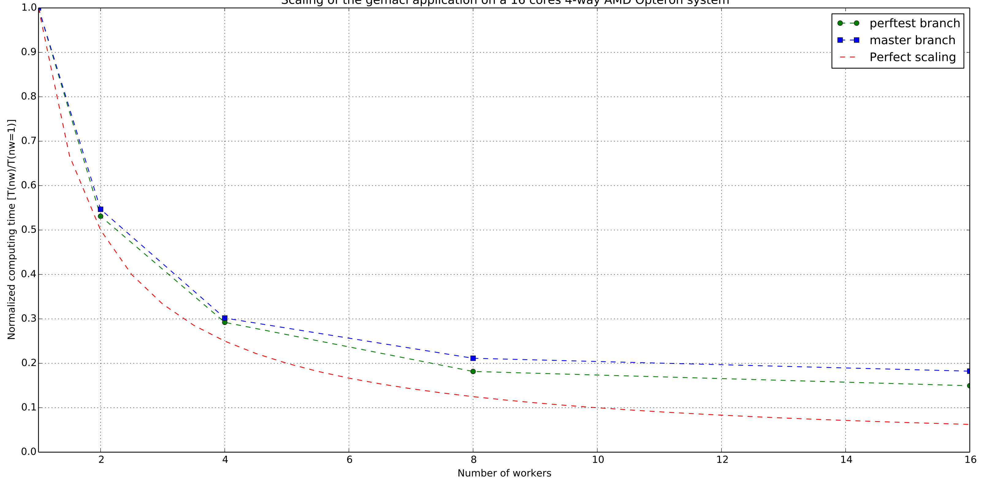
Scaling of the gemacl application on a 16 cores 4-way AMD Opteron system
