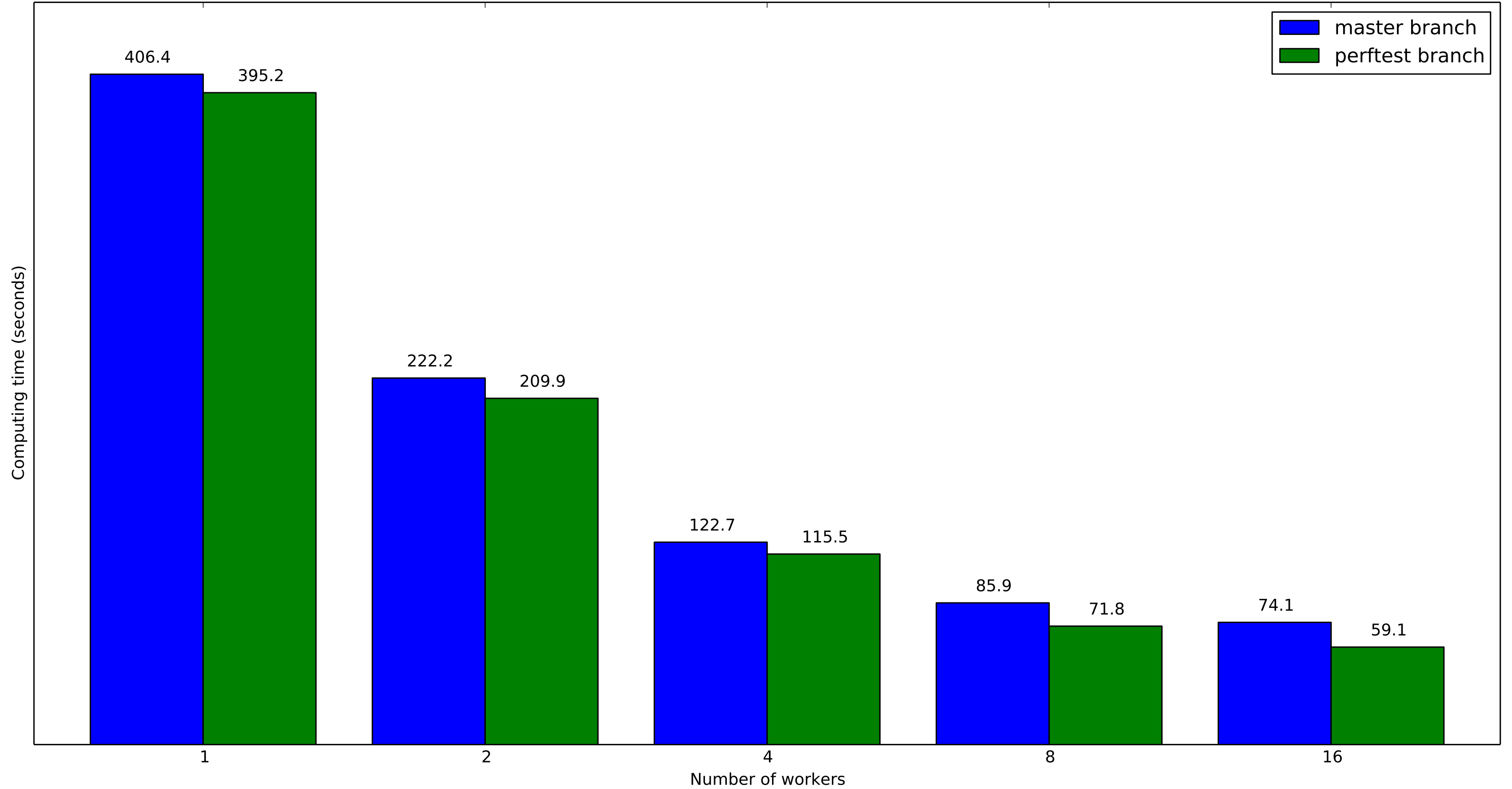
Computing times on a 16 cores 4-way AMD Opteron system
